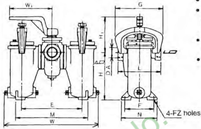
Model STW duplex strainer (diameter 12 - 40 mm)
