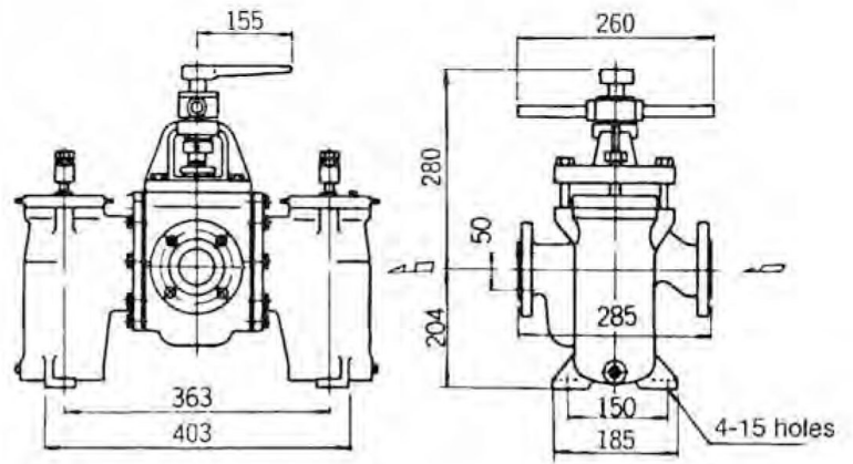
Direction of flow in model STW
