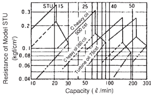
Model STU (single)
