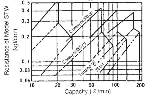
Model STW (duplex)
