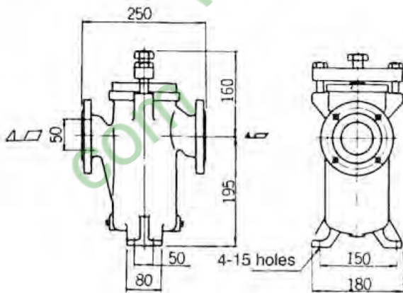
STU-50 (single): Flange JIS 10K
