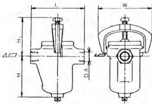
Model STU single strainer (diameter 12 - 40 mm)
