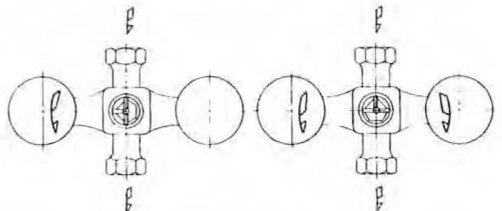
Direction of flow in model STW
